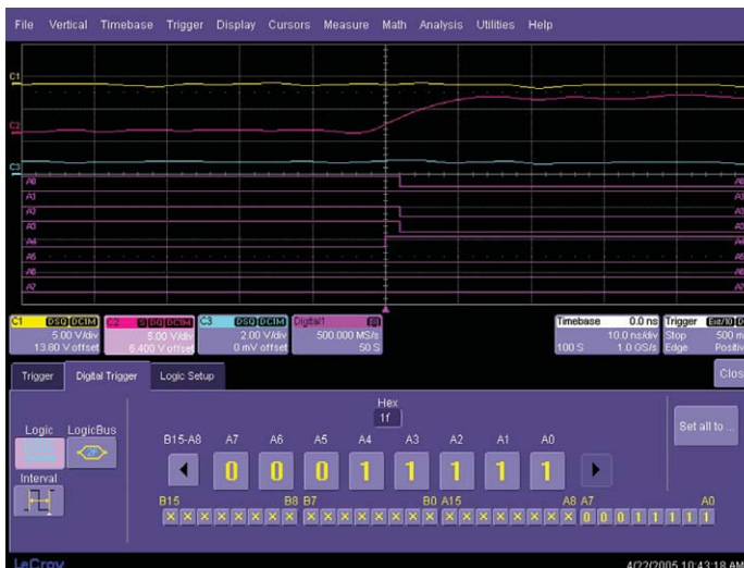
Figure 4. Without time-qualification, the scope triggers on unstable/transitional states (LeCroy WaveRunner with MSO option).
