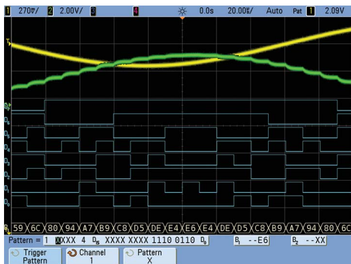
Figure 9. Agilent InfiniiVision Series MSO captures parallel digital input and analog output of MCU-controlled DAC.
