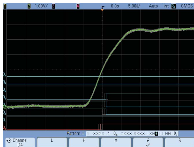
Figure 7. Real-time comparator hardware pattern triggering in an Agilent MSO generates very low trigger jitter.
