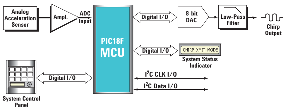
Figure 8. Mixed-signal embedded design that generates analog “chirp” outputs based on analog, digital, and serial I/O.
