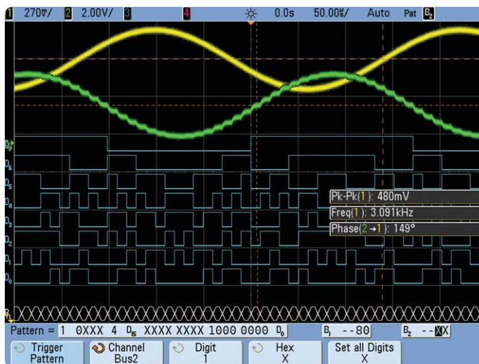
Figure 10. Agilent MSO triggers at the 50% crossing point using a combination of analog AND digital pattern triggering.
