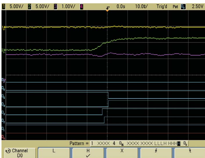
Figure 5. With minimum time-qualification, the Agilent MSO does not trigger on unstable conditions.
